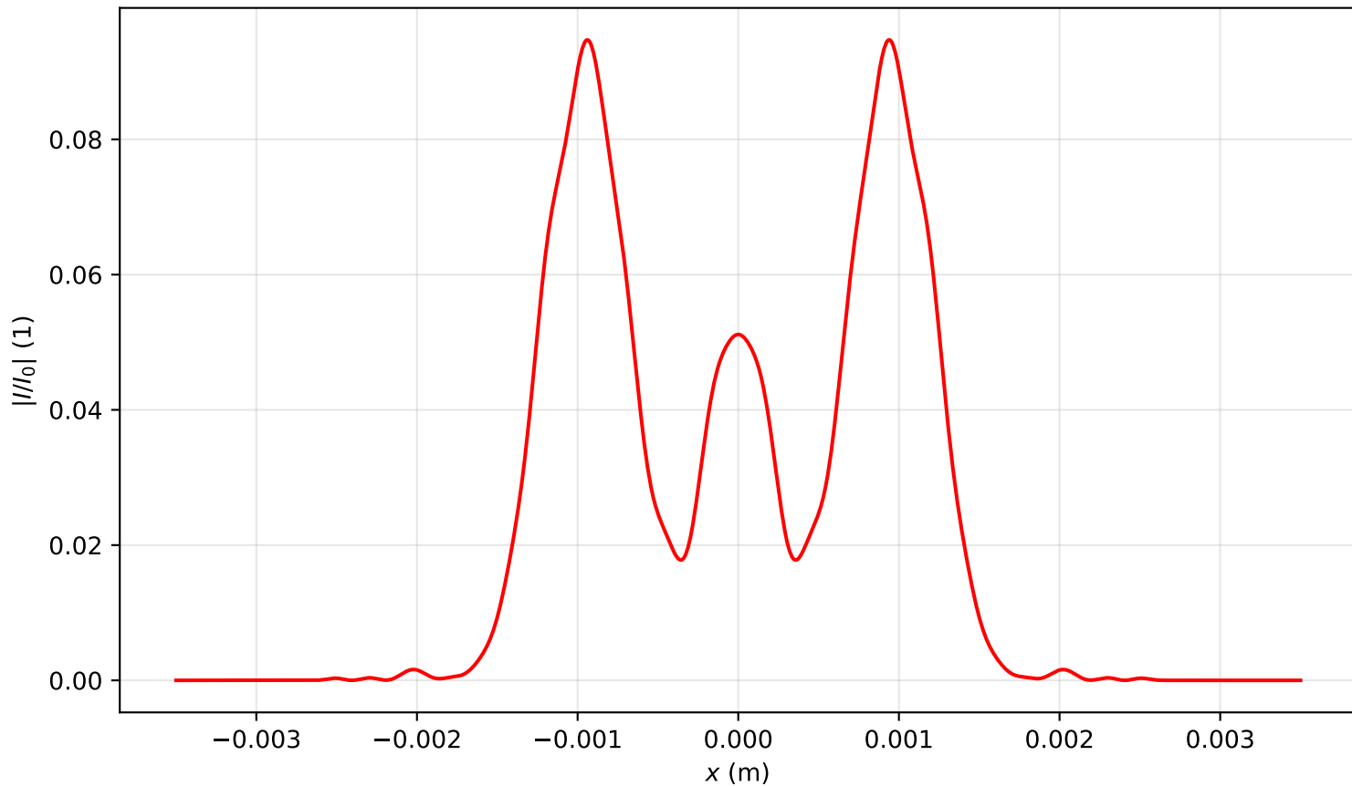
Intensity profile I(x, y = 0, z = 2.627)/I_0 , P_{in}=7.0P_{cr} , artificial time
